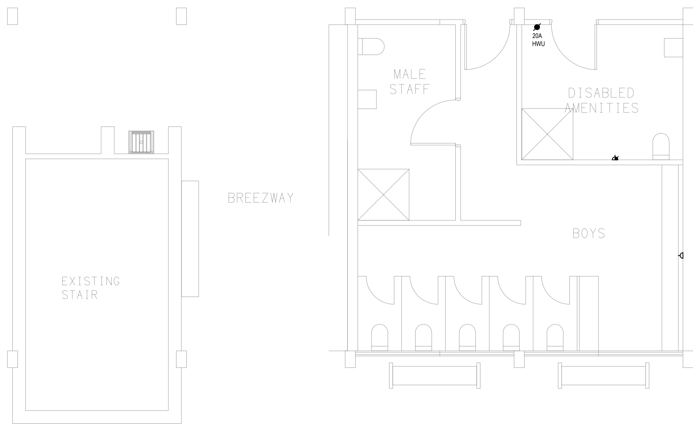
EXISTING / DEMOLITION POWER & COMMUNICATIONS LAYOUT SCALE 1:50
