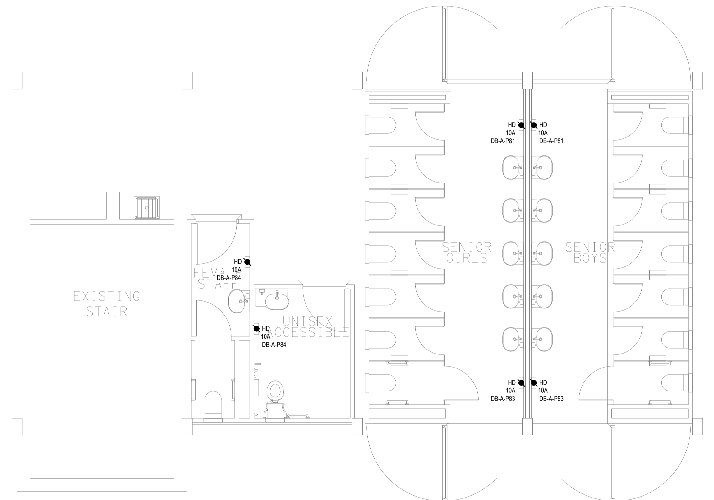
PROPOSED POWER & COMMUNICATIONS LAYOUT SENIOR STUDENTS SCALE 1:50
